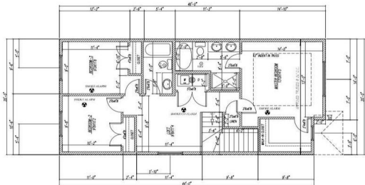
UPPER FLOOR PLAN 855 sq. ft.
