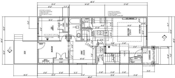
MAIN FLOOR PLAN 906 sq. ft.
